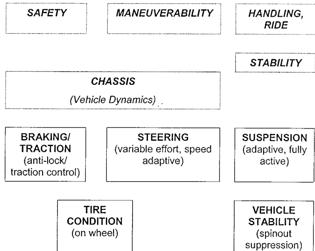
Fig. 3. Chassis systems, control functions and applications (Simplified diagram).
